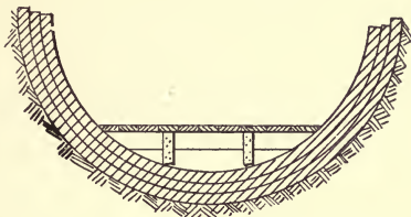
FIG. 24.—MASONS' PLATFORM FOR BRICK SEWERS.
